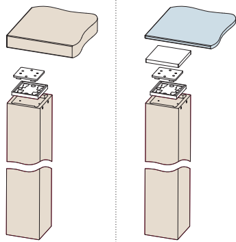
80x80 lesene noge / wooden legs
